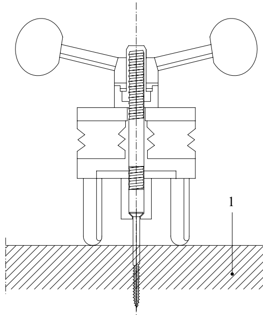
Figure 5: Principle of pull-out test assembly
