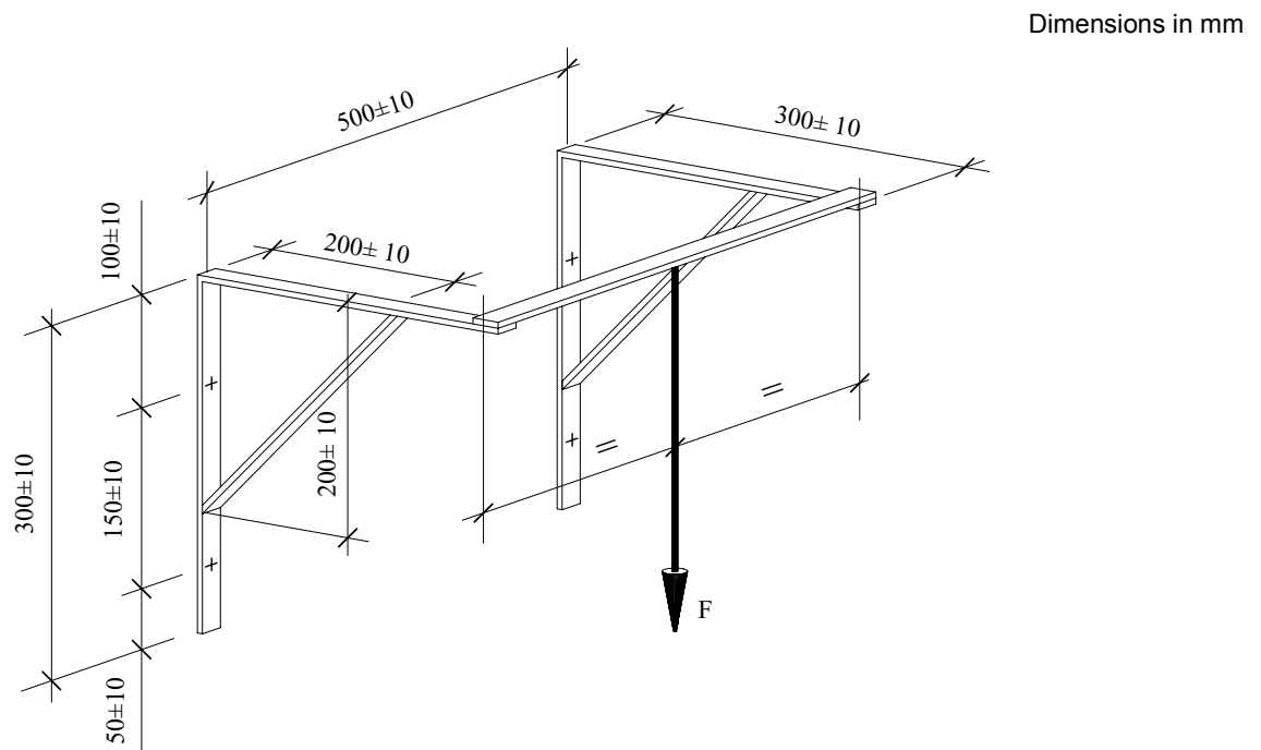
Figure 3: Principle of resistance to eccentric load test assembly
